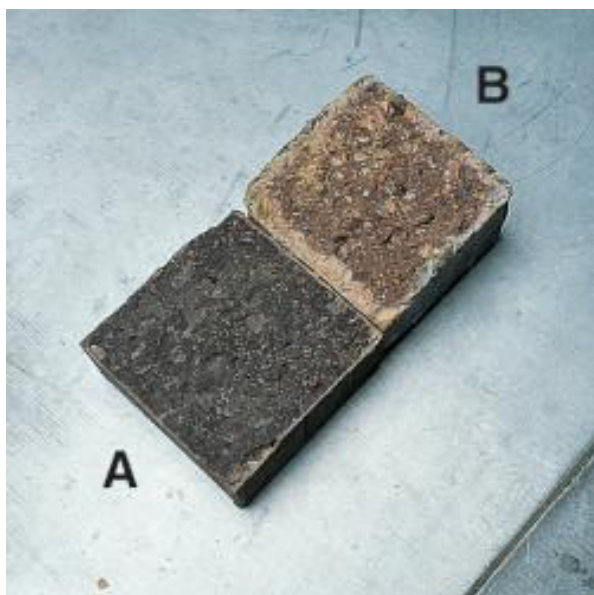
Fig. 2 B - Chloride ion penetration tests (UNI 9944). Specimen A, coated with Mapelastic Zero , appears to be unpenetrated; specimen B, as-is, shows an advanced penetration of several millimetres
