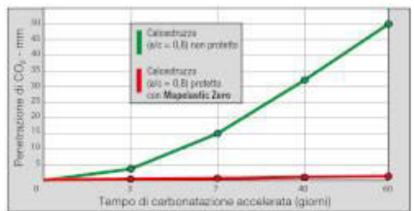
Fig. 2: Effect of Mapelastic Zero on accelerated carbonation (30% CO 2 ) in a porous concrete
