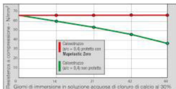
Fig.4: Effect Mapelastic Zero on the reduction in mechanical strength of concrete due to calcium chloride de-icing salts
