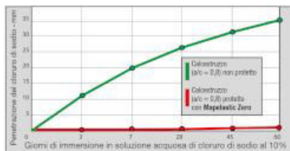
Fig.3: Effect of Mapelastic Zero on the penetration of sodium chloride into a porous concrete
