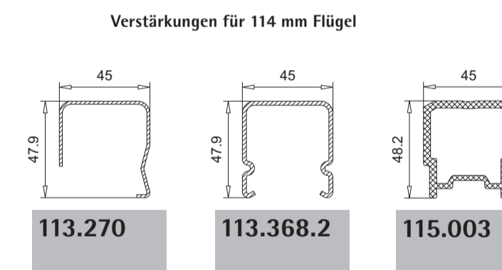
113.270 113.368.2 115.003
